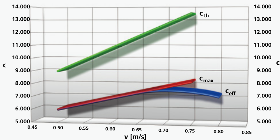
Transportation capacity c (persons/h) as a function of speed
