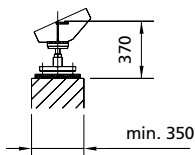
Detail Y (two or more intermediate supports)
